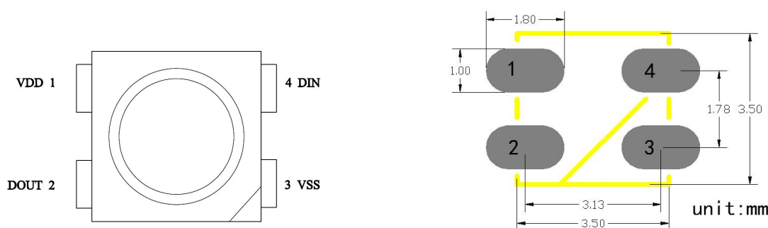
Recommended PCB size
