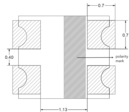
PCB Solder Pad
